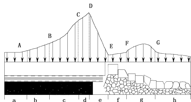
Fig. 1. Distribution of pressure on roofs at the front and back of the stope face:
