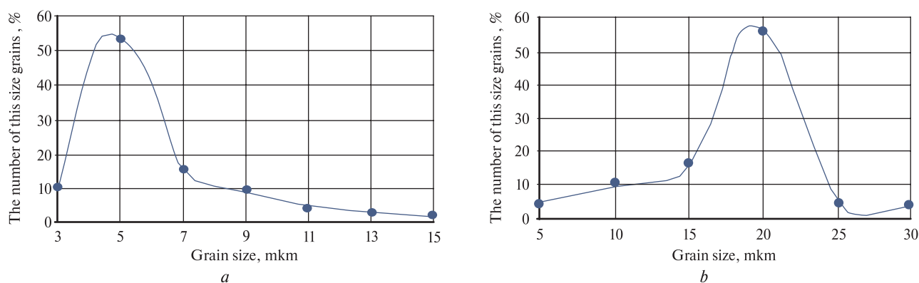
Fig. 6. Grain distribution in terms of their size in the cement stone samples:
