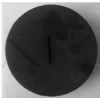
Fig. 3. SNBD Specimen made by high-pressure water jet method
