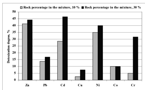
Fig. 1. The ash detoxication degree provided by carbonate clay
